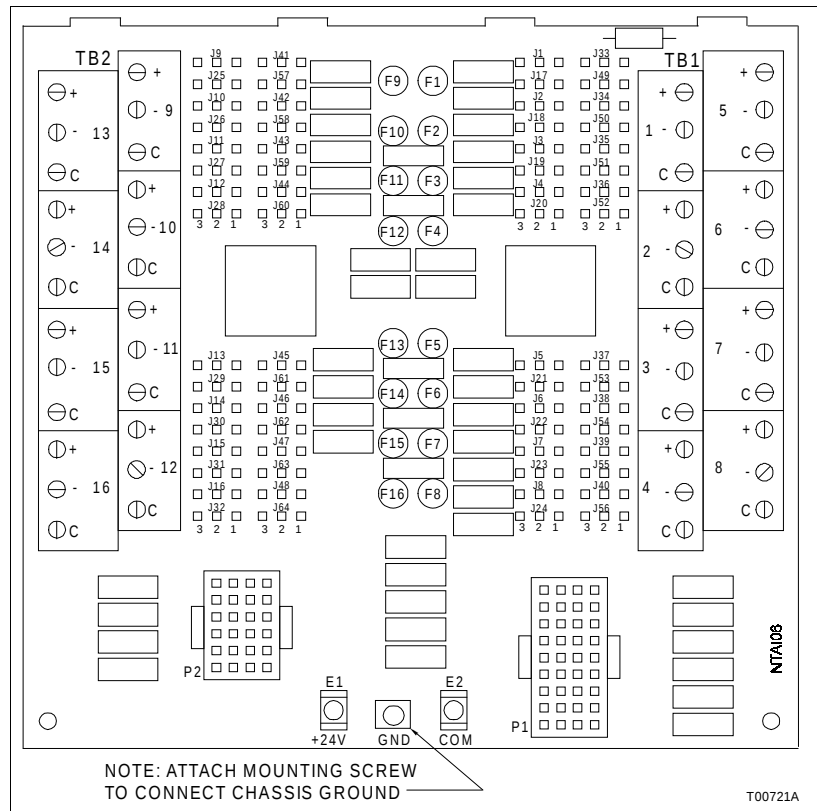
Figure 2-2. Jumper Locations and Terminal Assignments for NTA106 Revision B Hardware (6639364B1)
