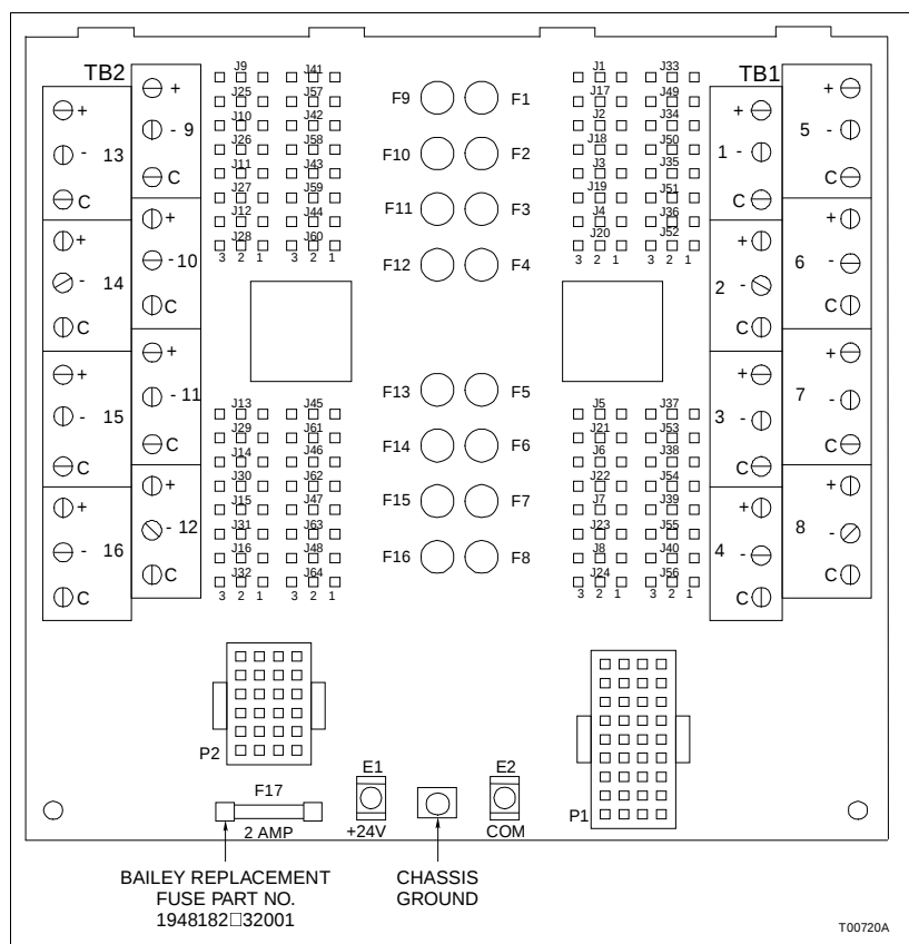
Figure 2-1. Jumper Locations and Terminal Assignments for NTAI06 Revision A Hardware (6639364A1)
