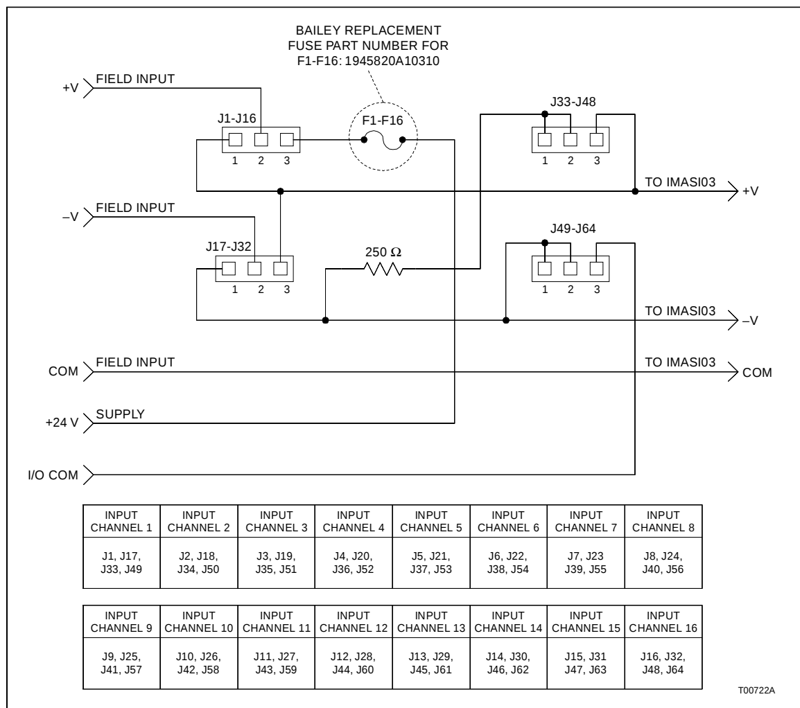
Figure 2-3. Typical Input Circuit for NTAIO6
