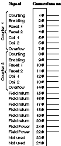
AS-B882-239 Terminal Numbering and Wire Connections
