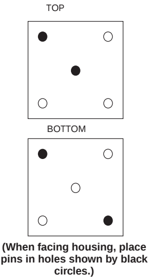
AS-B882-239 Mechanical Keying for Housings
