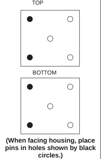
AS-B809-016 Mechanical Keying for Housings
