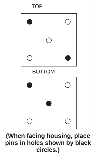
AS-B863-032 Mechanical Keying for Housings
