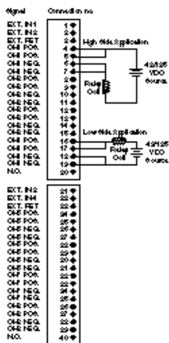
AS-B881-508 Terminal Numbering and Wire Connections
